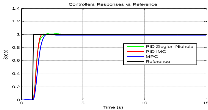
Figure 7: Controllers' Unit Step Responses Comparison
