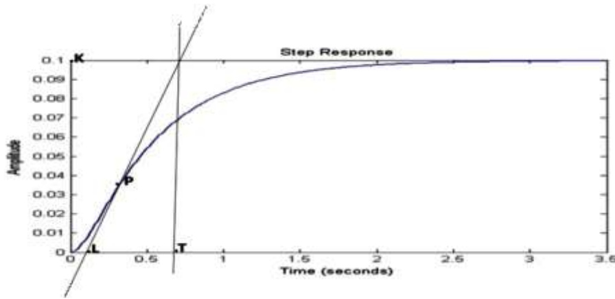
Figure 3. Step response of the motor open-loop plant showing FOPDT parameters [12].
