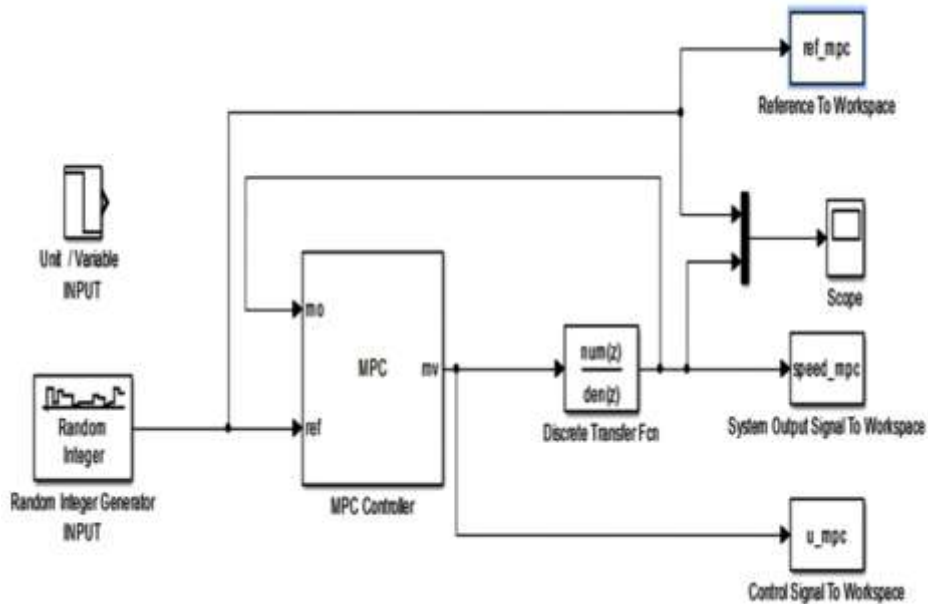
Figure 6: MPC model structure [16]
